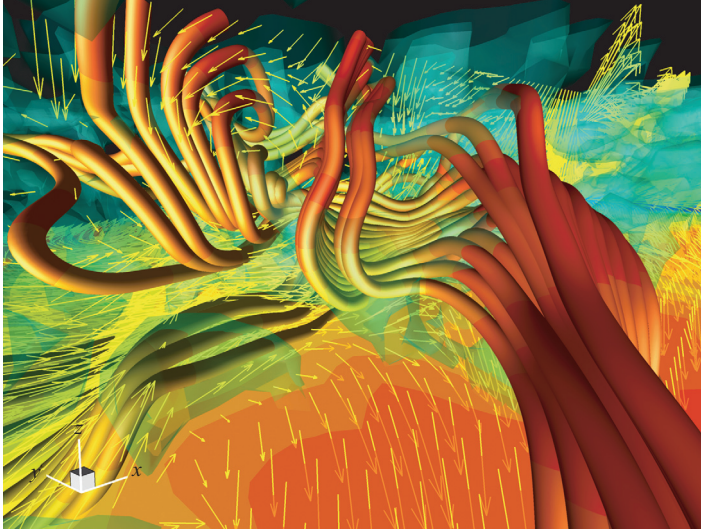
FIGURE 12. Instantaneous flow structure of the incoming boundary layer: upper region ( z/\delta = 0.6\text{--}1.0 ). Semitransparent vorticity magnitude isosurfaces for |\boldsymbol{\omega}|\delta/U_\infty = 0.5 are shown. Velocity vectors with a convective velocity of 0.8U_\infty are shown in two planes; at y/\delta = 0.5 and z/\delta = 0.6 , the latter flooded with streamwise velocity contours. Streamlines are computed within this convective reference frame.
