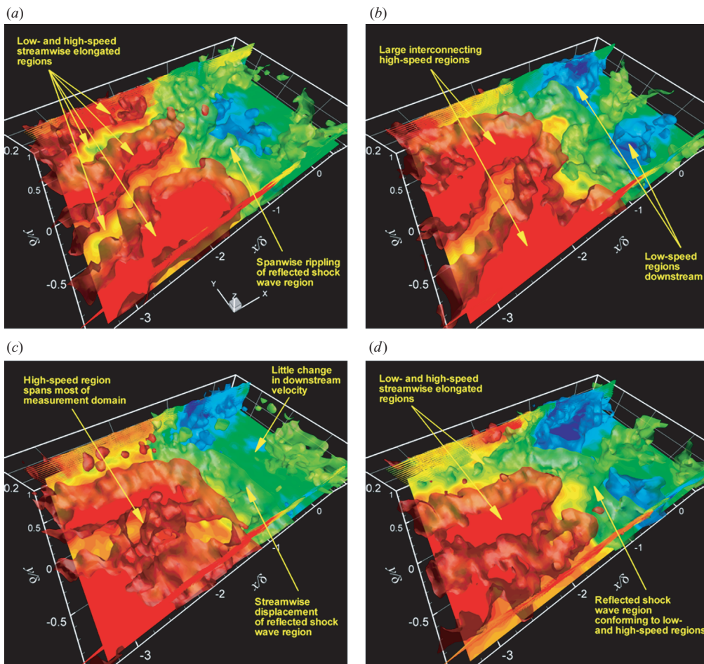
FIGURE 8. Volumetric representations of the instantaneous flow organization of the interaction: lower region ( z/\delta = 0.1\text{--}0.6 ). Isosurfaces of streamwise velocity are shown: relatively high-speed in red ( 0.9U_\infty ), intermediate velocity in green ( 0.75U_\infty ), and relatively low-speed in blue ( 0.55U_\infty ). Velocity vectors are shown flooded with instantaneous streamwise velocity. (a, b) correspond to figure 7 (a, b).
